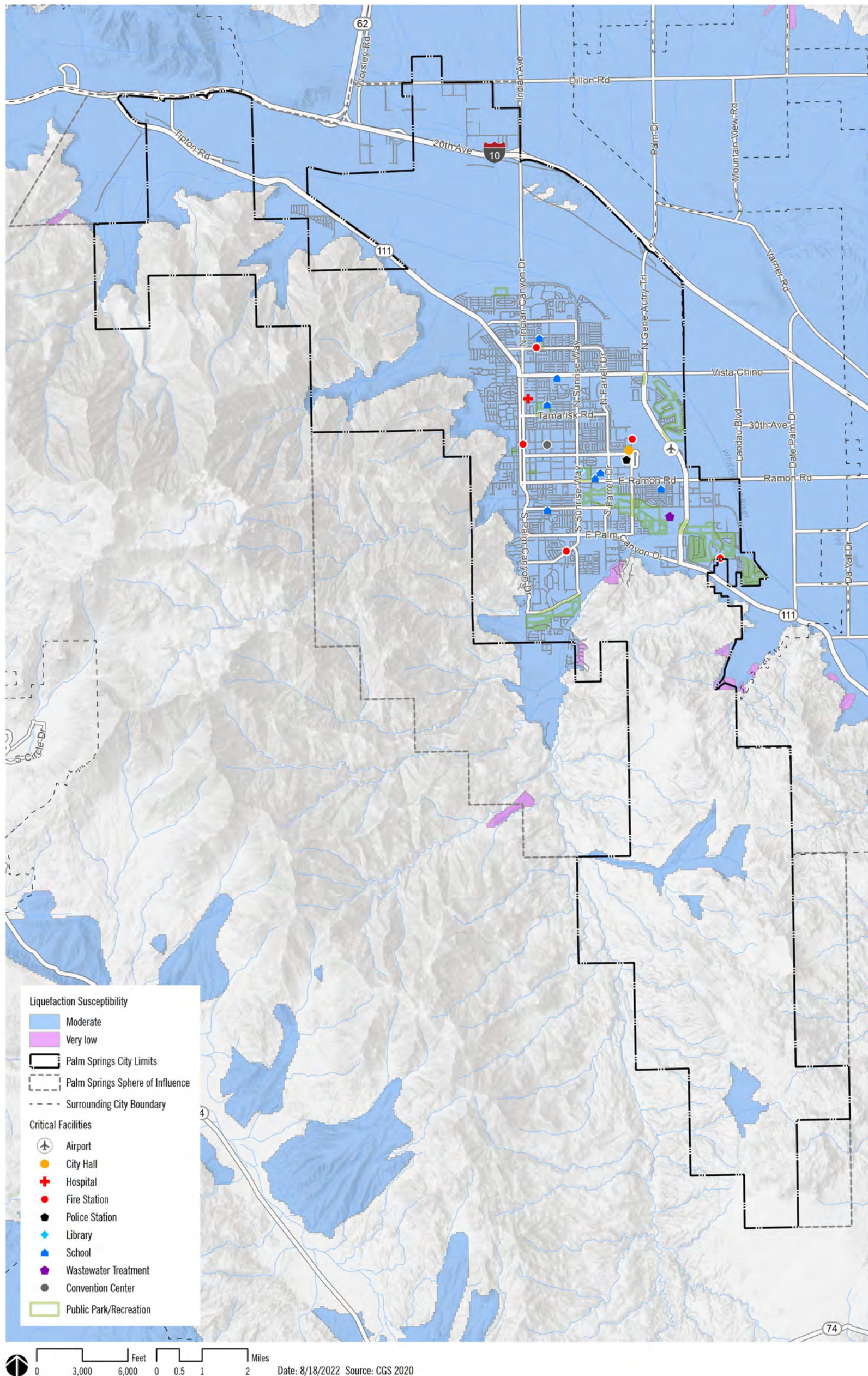
Figure 6-3 Liquefaction Potential
