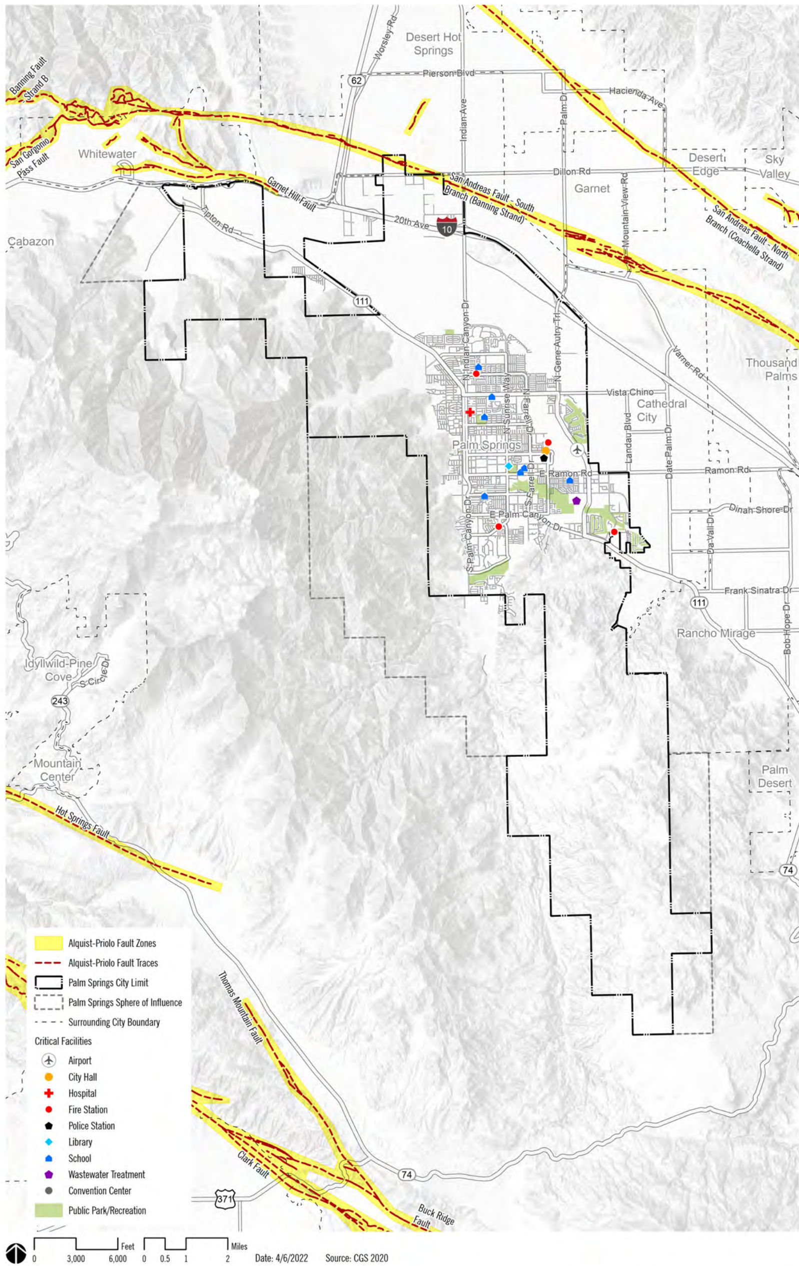
Figure 6-2 Regional Faults
